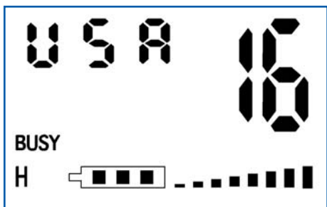
Fig. 2: Busy Indicator
